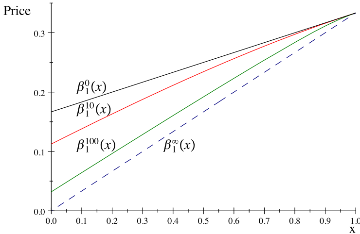
Fig. 2. Round 1 equilibrium bids for N = 3 , U[0, 1] , and \alpha = 0, 10, 100 , and \infty .
