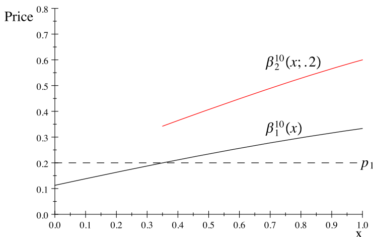
Fig. 1. Equilibrium bids by round, for N = 3 , U[0, 1] , and CARA(\alpha = 10) .
